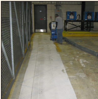
Shot Blasting
